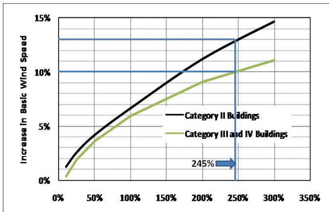
2 Percentage increase in basic wind speed in St. Lucia vs. percentage increase in annual rates of Category 4 and 5 hurricanes. Based on work of Dr Peter Vickery of Applied Research Associates
