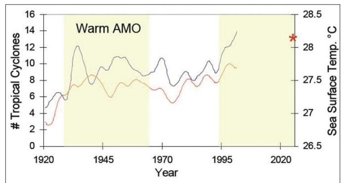
1 North Atlantic Tropical Cyclones & SST – Decadal scale variations: 9-yr Hamming filter. (Courtesy of Judith Curry, Georgia Institute of Technology)
