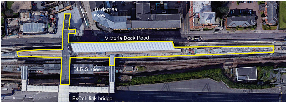
Figure 2 Plan of Custom House station showing 18° skew of site derived from 'urban grain' (relationship between Freemasons Road and Victoria Dock Road)
