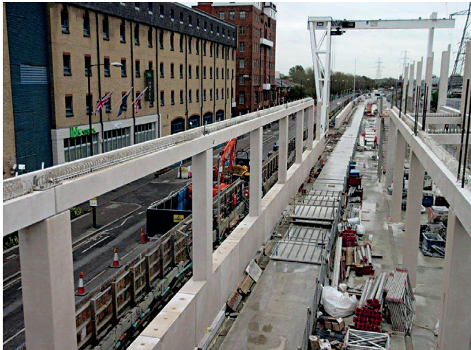
➔ Figure 14 Precast panels with triangular vaulted soffits are used on main span of concourse structure
