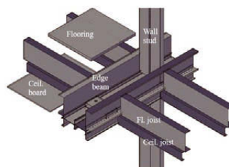
(a) Typical CFS modular framing
