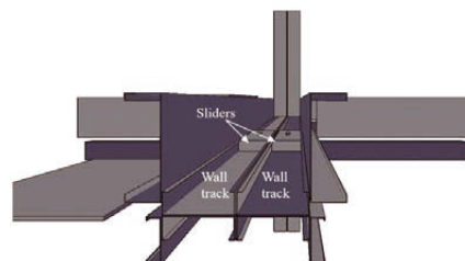
(b) Slider devices in wall tracks of neighbouring modules
