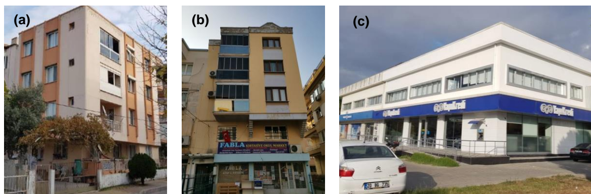
Figure 80: Good response of (a) – (b) RC frames with infill masonry walls and (c) RC precast industrial building
