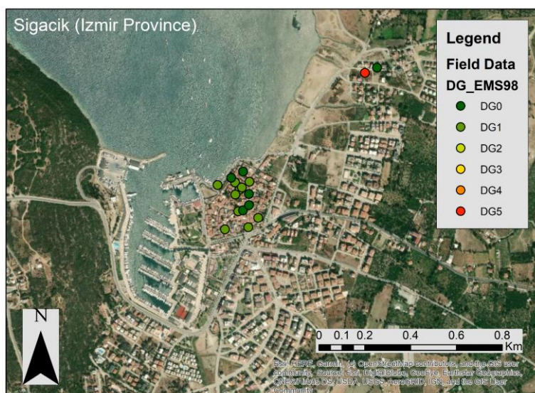
Figure 104: Damage assessment data for surveyed buildings in Sığacık.
