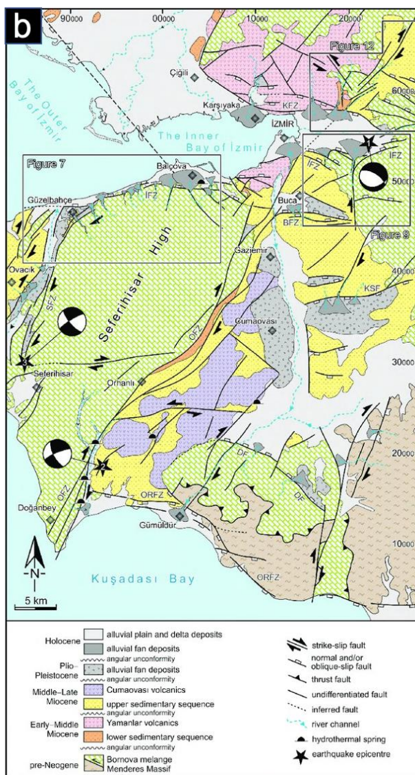
Figure 4: (a) Geological map for the Island of Samos (Ring et al., 2007) and (b) geology for the area SW of the city of Izmir (Uzel et al., 2009)
