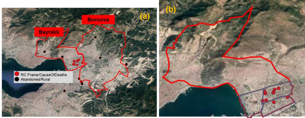
Figure 83: Map of collapsed buildings in Bayraklı and Bornova (21) and (b) location of the RC frame buildings in Bayraklı
