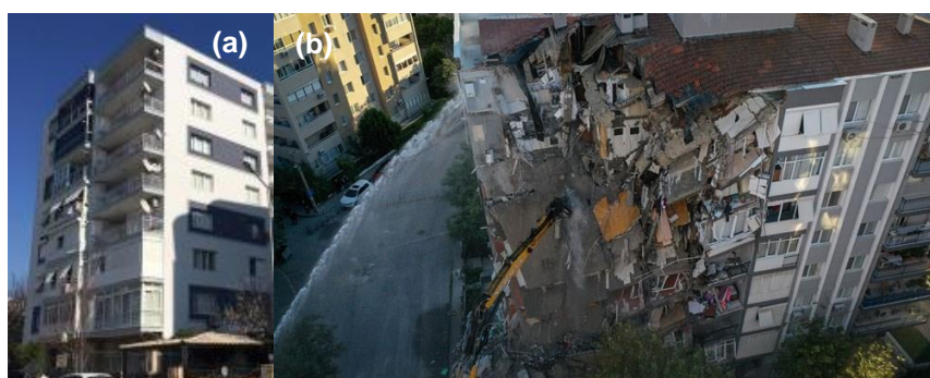
Figure 86: Karagül Apartments: (a) before ( http://puzzleyapi.com/karagul-apt-bayrakli-izmir/ ) and (b) after the earthquake ( https://www.birgun.net/haber/coken-karagul-apartmani-na-da-10-yil-once-rapor-verilmis-321551 )
